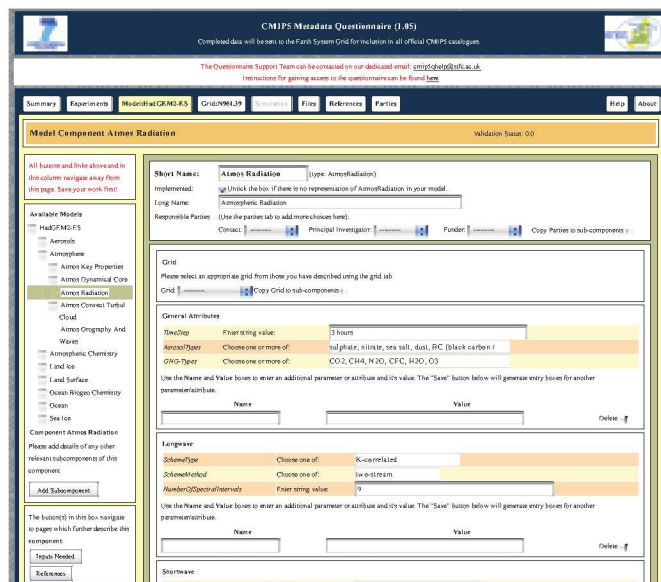
Figure 3: Screen shot of the CMIP5 questionnaire. This screen shot shows part of the entry form for describing the longwave atmosphere radiation scheme; it is generated from the mind map shown in Figure 2.
